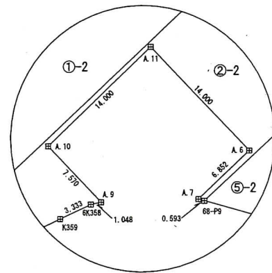
拡大図D S=1:500
