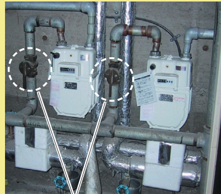
main valve
